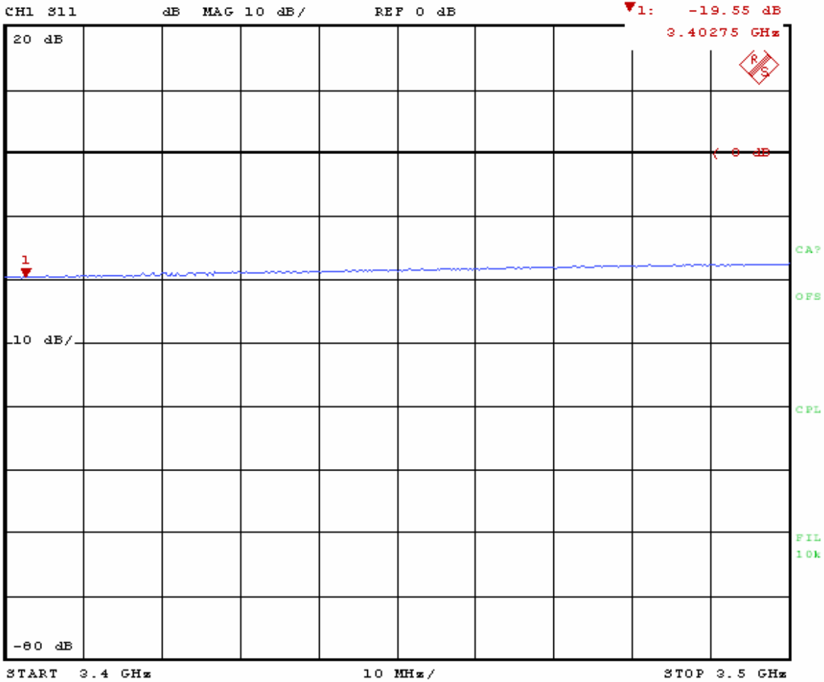
SWR Reflection input port 1
